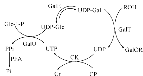
Scheme 3. CUPE Cycle with CP-CK Regeneration System a
