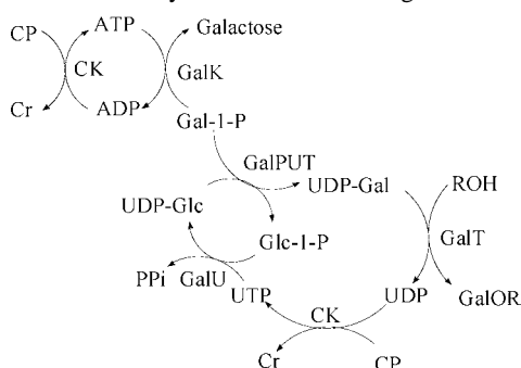
Scheme 2. KTCU Cycle with CP-CK Regeneration System a
