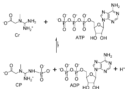
Figure 1. Creatine kinase reaction.
