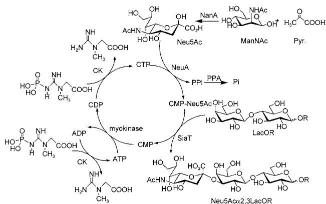
Scheme 1. Sialylation Cycle with CP–CK Regeneration System
